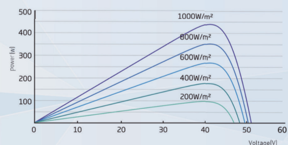
P-V Curve at Different Irradiation (440W)
