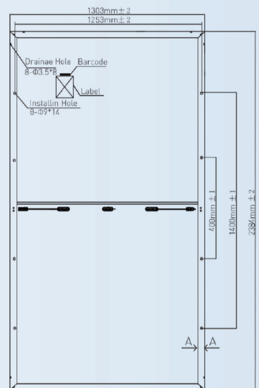
Back View
